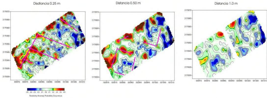
Figure 4. Geoelectrical maps.
