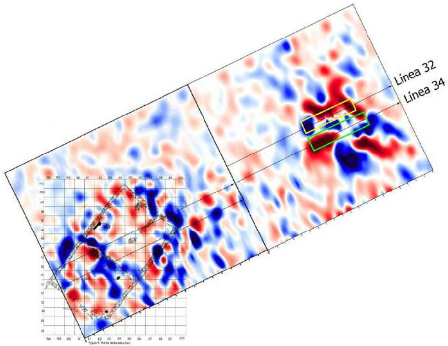
Figure 13. Georadar verification of magnetic anomalies.
