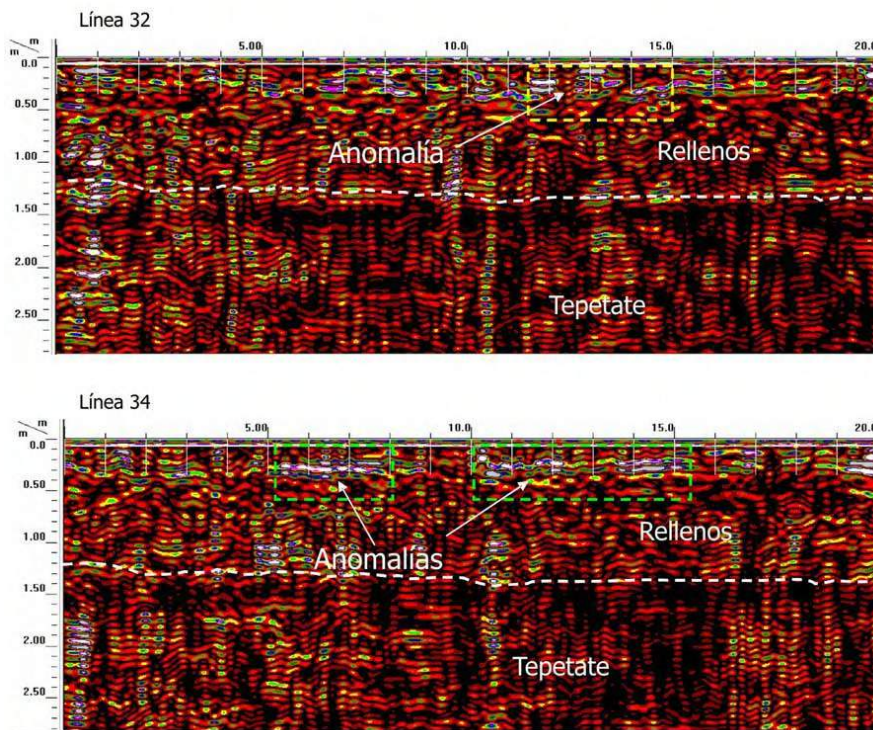
Figure 14. Radargrams of the circular anomaly.
